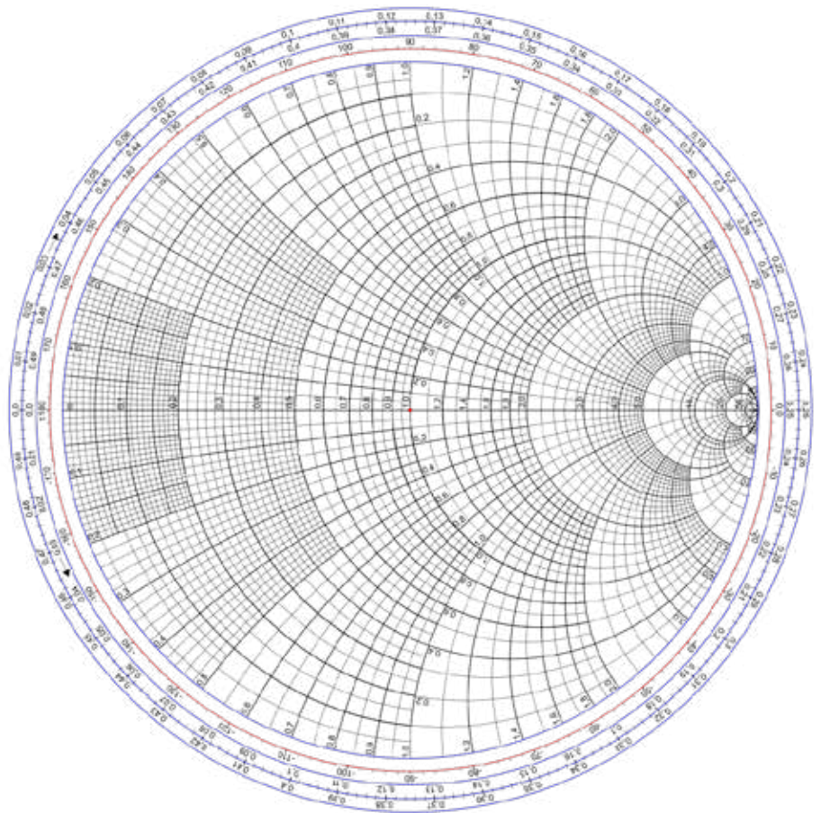
Fig 1. Smith Chart
