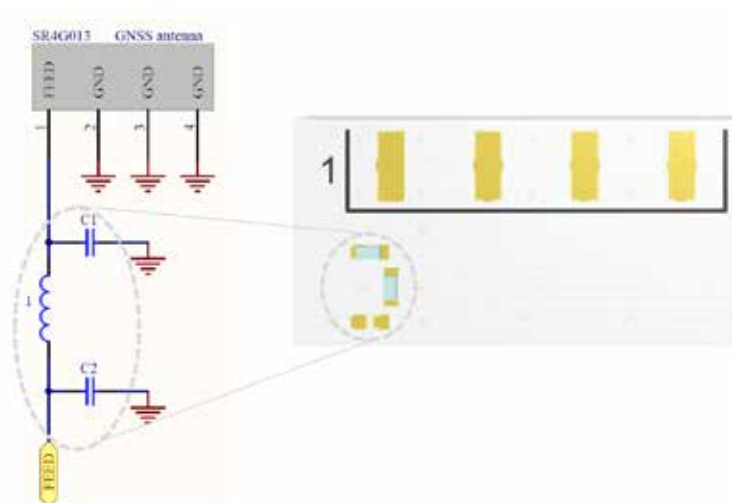
Fig 2. Pi Matching Network Example for Antenova SR4G013 'Beltii'
